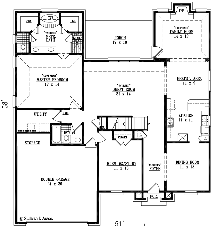
FIRST LEVEL FLOOR PLAN
